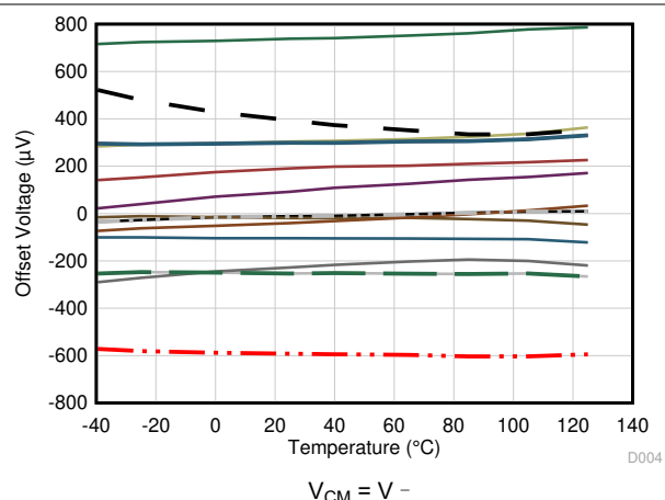
图 6-2. Offset Voltage Drift Distribution
