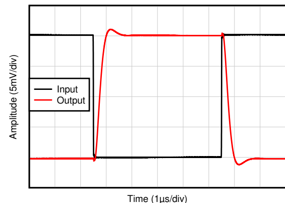
图 6-34. Negative Overload Recovery
