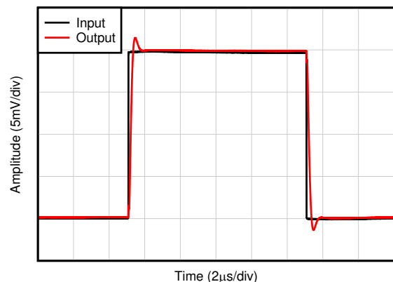
图 6-33. Positive Overload Recovery
