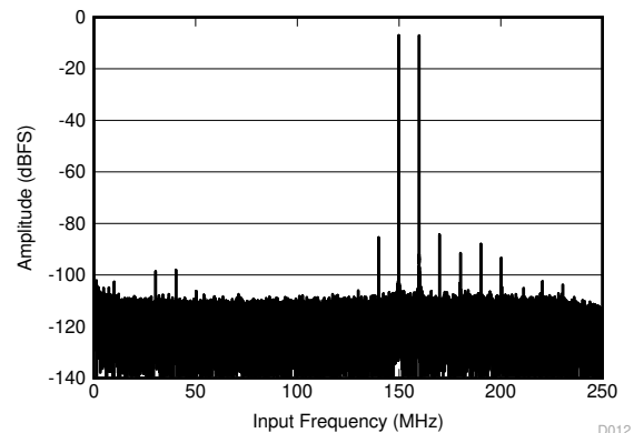
图 6-11. FFT for Two-Tone Input Signal
