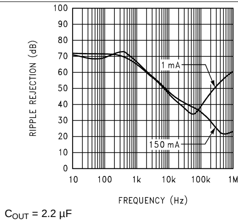
Figure 13. Ripple Rejection
