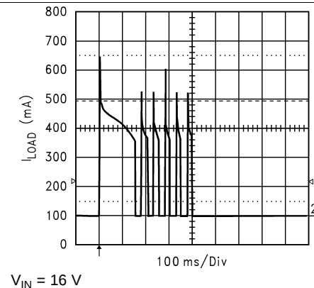
Figure 14. Turnon Time
