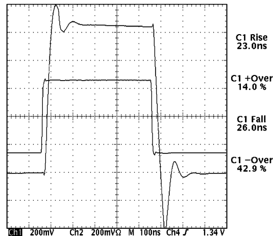
Figure 56. R_C = 240\Omega and C = 2.2 \text{ nF} , Gain = +2
