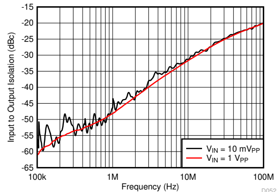
图 6-24. Input-to-Output Disable Mode Isolation
