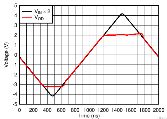
图 6-33. Input Overdrive Recovery
