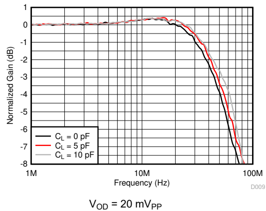
图 6-21. Small-Signal Frequency Response Over C_L
