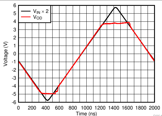
图 6-29. Input Overdrive Recovery
