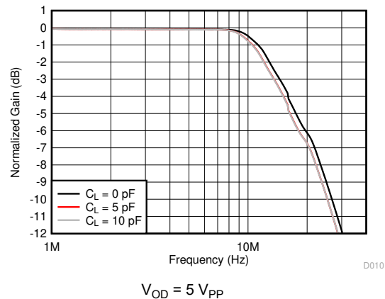
图 6-22. Large-Signal Frequency Response Over C_L
