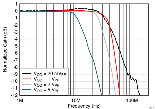
图 6-23. Frequency Response Over Differential Output Voltage, V_{OD}
