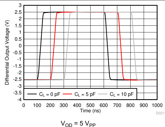
图 6-28. Large-Signal Step Response Over C_L
