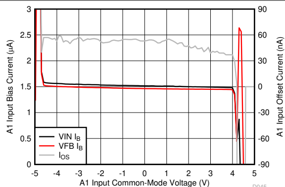
图 6-14. A1 Input Bias Current and Input Offset Current vs Input Common-Mode Voltage
