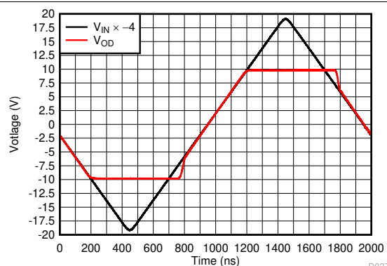
图 6-18. Output Overdrive Recovery
