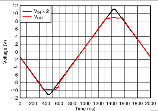
图 6-17. Input Overdrive Recovery
