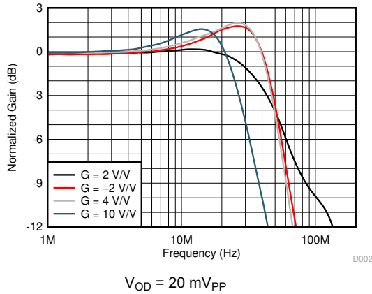
图 6-19. Small-Signal Frequency Response
