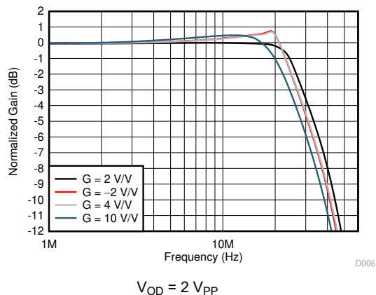
图 6-32. Large-Signal Frequency Response
