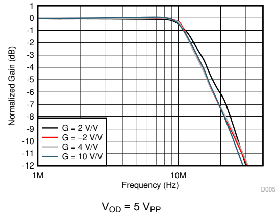
图 6-20. Large-Signal Frequency Response
