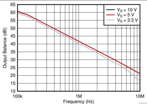
图 6-45. Output Balance vs Frequency
