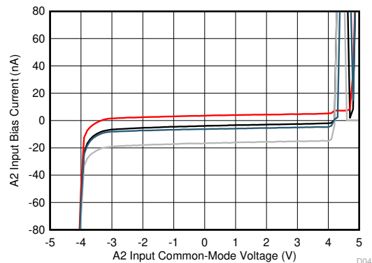
图 6-16. A2 Input Bias Current vs Input Common-Mode Voltage
