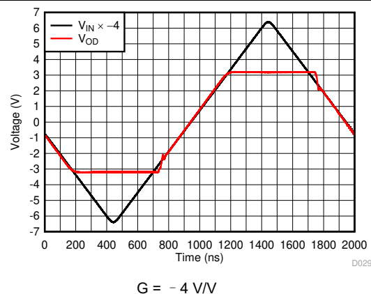
图 6-34. Output Overdrive Recovery
