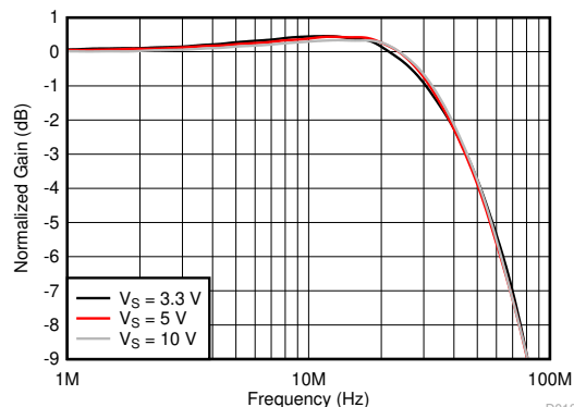
图 6-36. V_{REF} Small-Signal Frequency Response
