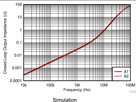
图 6-6. Closed-Loop Output Impedance vs Frequency
