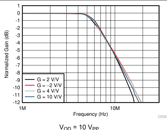
图 6-2. Large-Signal Frequency Response
