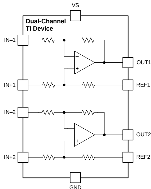
图 40. INA2181 Functional Block Diagram
