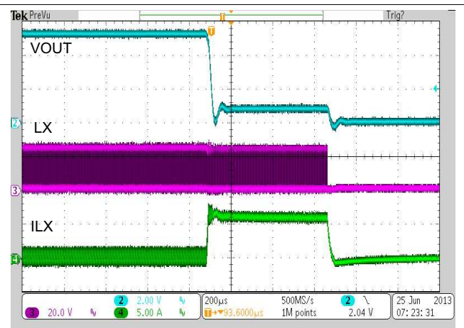
Figure 45. Buck Output Hard Short Response (Zoom In)
