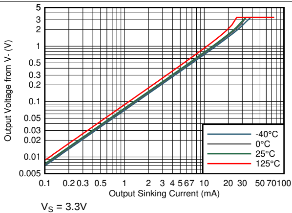
图 25. Output Voltage vs Output Sinking Current
