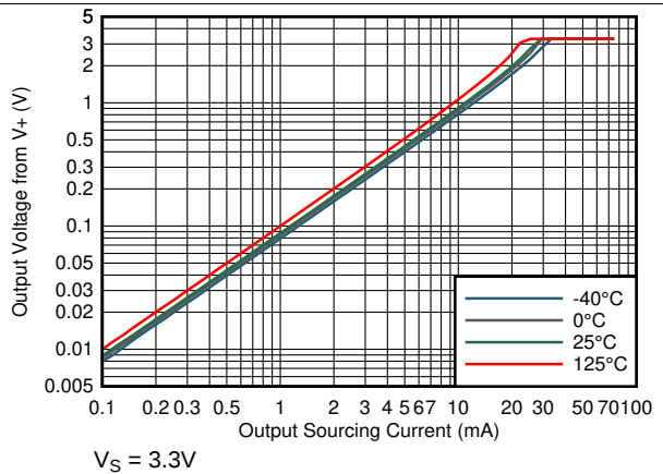
图 26. Output Voltage vs Output Sourcing Current
