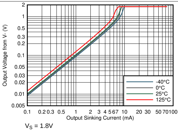
图 23. Output Voltage vs Output Sinking Current
