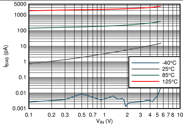
图 21. Bias Current vs Common Mode Voltage
