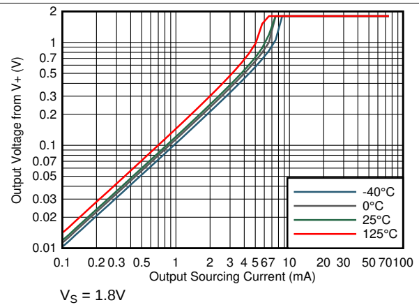
图 24. Output Voltage vs Output Sourcing Current
