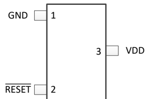
DBZ Package (Pin 1 = GND) 3-Pin SOT-23 Top View
