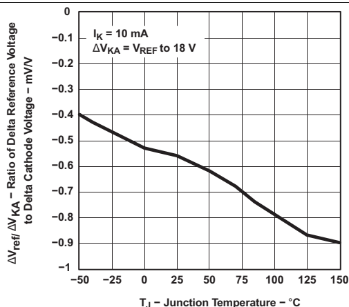
Figure 7. Ratio of Delta Reference Voltage to Delta Cathode Voltage vs Junction Temperature
