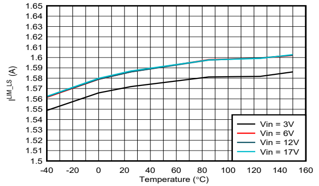
图 7-14. Low-Side I_{LIM} vs Temperature
