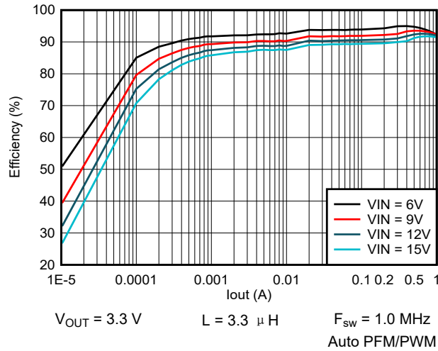
图 9-20. Efficiency vs Output Current
