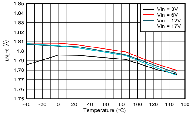
图 7-13. High-Side I_{LIM} vs Temperature
