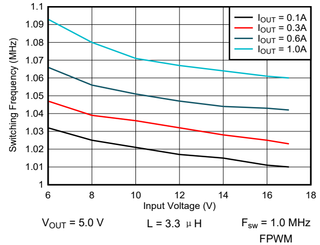
图 9-11. Switching Frequency vs Input Voltage
