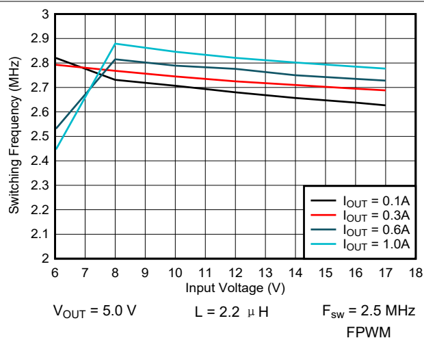
图 9-5. Switching Frequency vs Input Voltage
