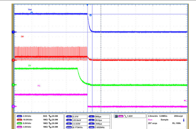
图 9-65. Shutdown Timing with Output Discharge Enabled
