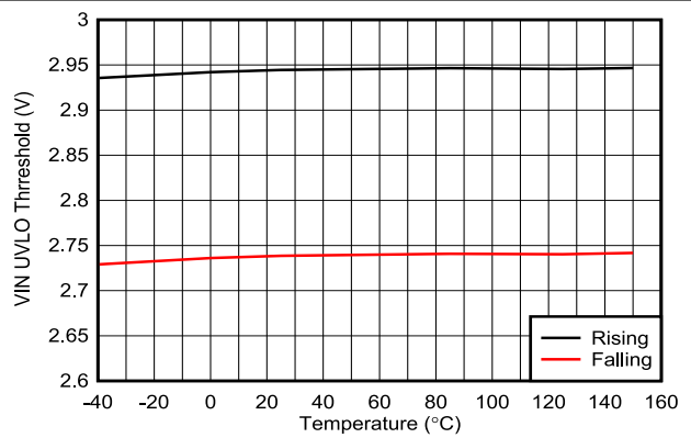
图 7-16. V_{IN} UVLO Thresholds vs Temperature
