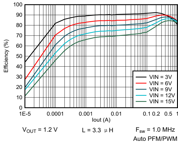
图 9-44. Efficiency vs Output Current
