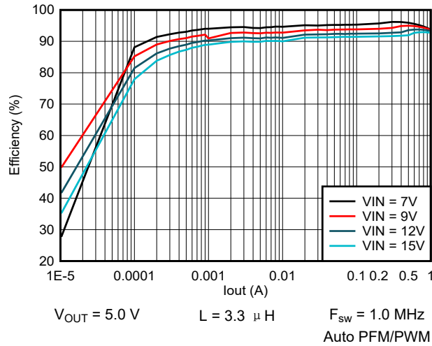
图 9-8. Efficiency vs Output Current
