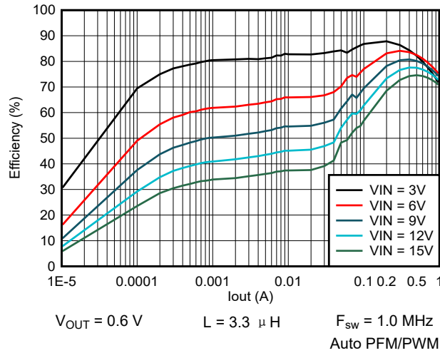
图 9-56. Efficiency vs Output Current
