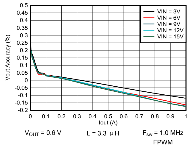
图 9-61. Output Voltage vs Output Current
