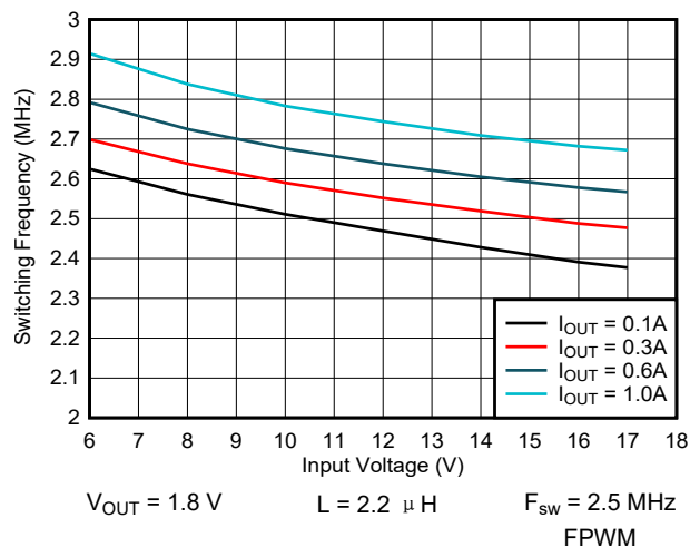
图 9-29. Switching Frequency vs Input Voltage
