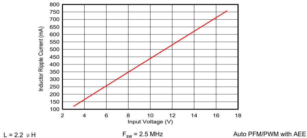
图 8-4. Typical Inductor Ripple Current Versus Input Voltage in AEE mode
