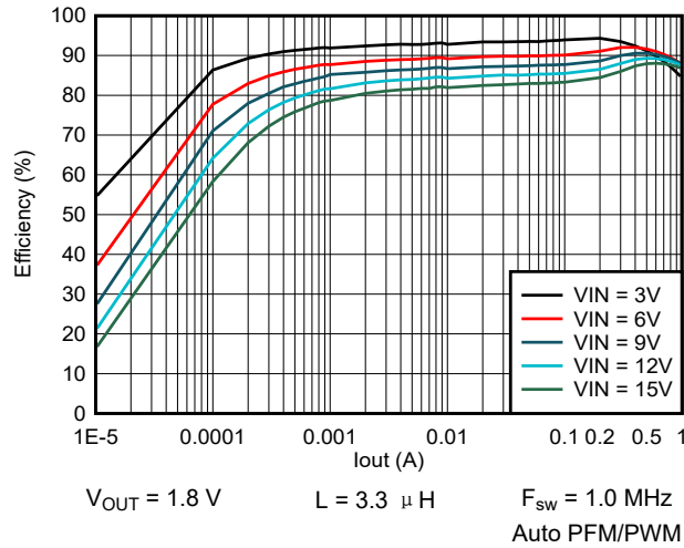
图 9-32. Efficiency vs Output Current
