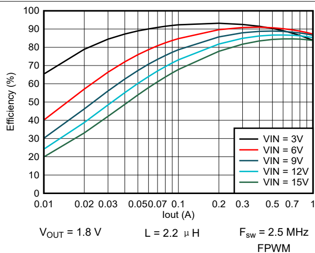
图 9-27. Efficiency vs Output Current
