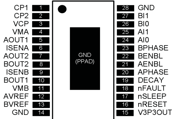
Pin Functions
