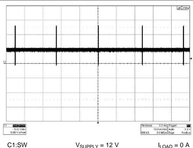
Figure 46. Skip Cycle
