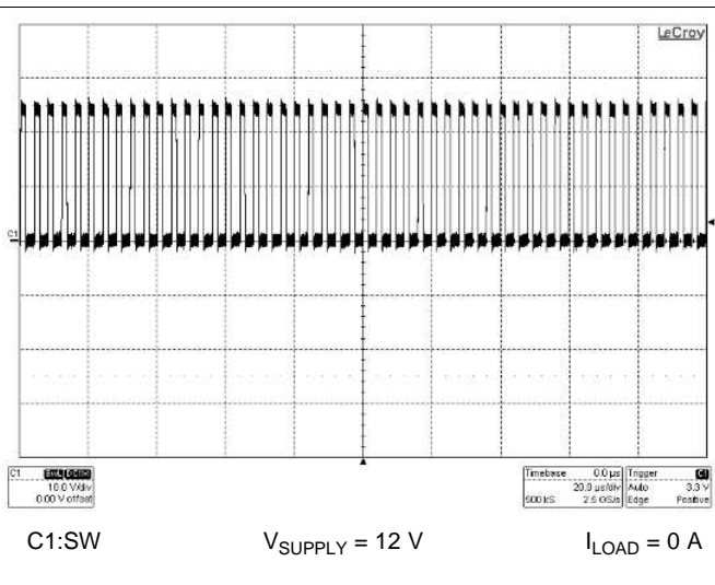
Figure 44. Forced PWM
