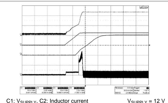
Figure 46. Skip Cycle
