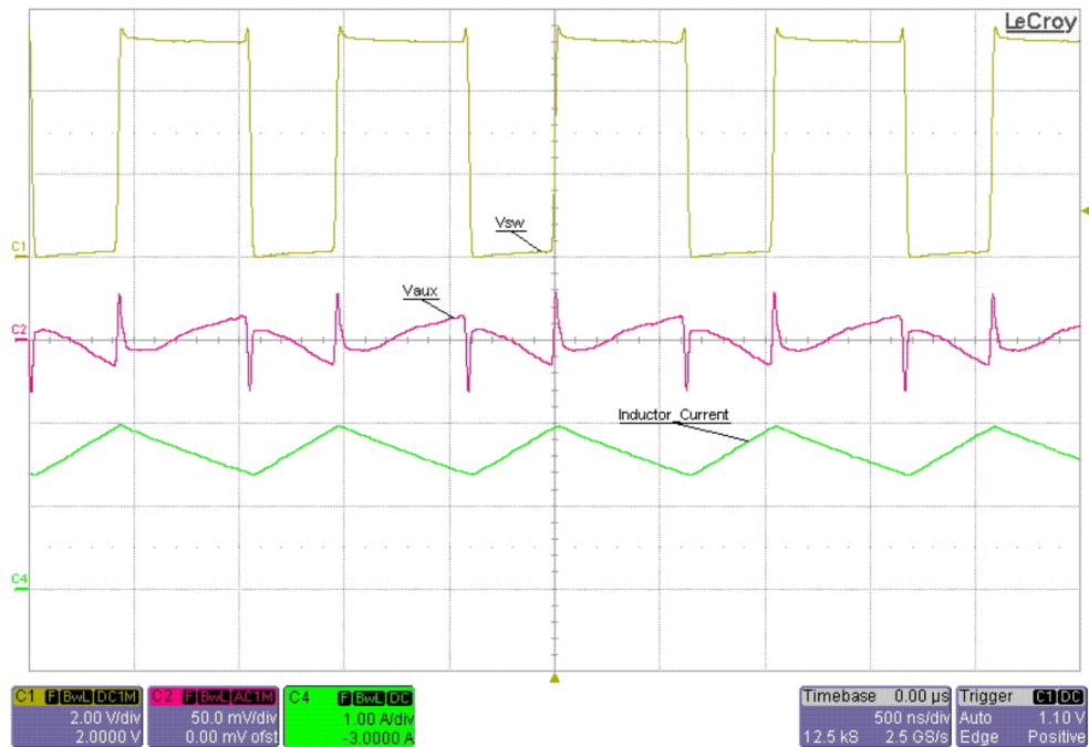
Figure 29. V AUX Ripple, V IN = 3.3 V, I AUX = 1 A
