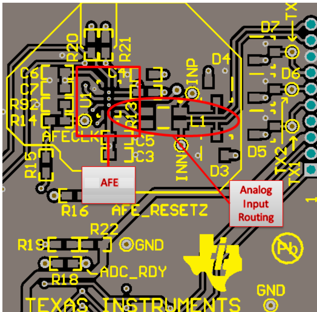
Figure 98. Example Layout
