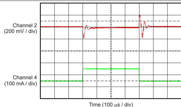
Figure 18. TPS70612 Load Transient (50 mA to 150 mA)
