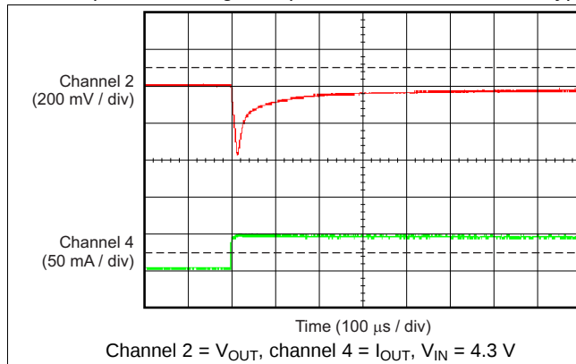
Figure 19. TPS70633 Load Transient (0 mA to 50 mA)
