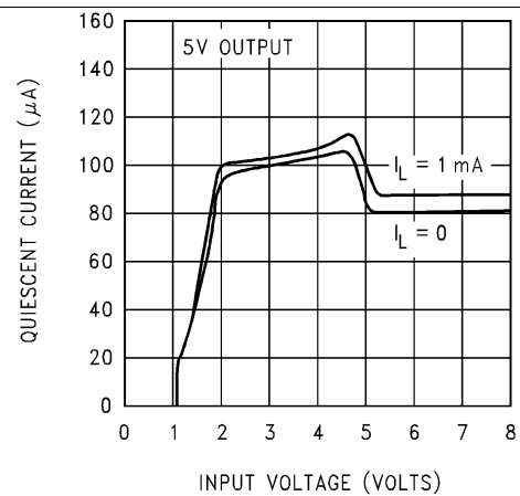
Figure 6. Quiescent Current
