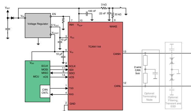
Simplified Schematics
