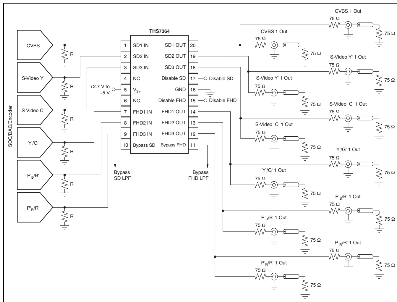
(1) Figure 81. Typical Six-Channel System with DC-Coupled Line Driving and Two Outputs Per Channel
