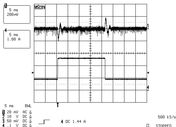
Figure 10-8. Output Voltage During 0.9-A to 2.7-A Load Transient (CH1: Output Voltage AC Coupled, 200 mV/div; CH4: Output Current, 1 A/div)
