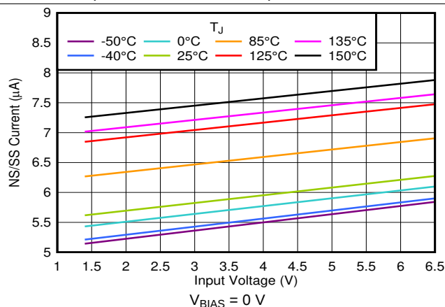
图 32. NR/SS Current vs Input Voltage and Temperature
