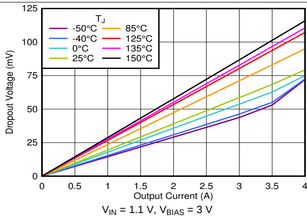
图 23. Dropout Voltage vs Output Current With Bias
