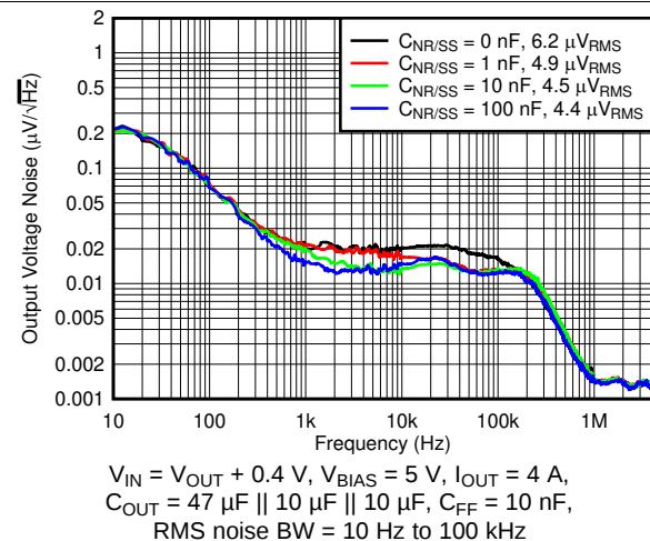
图 12. Output Noise vs Frequency and C_{NR/SS}
