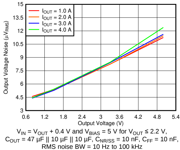
图 9. Output Voltage Noise vs Output Voltage
