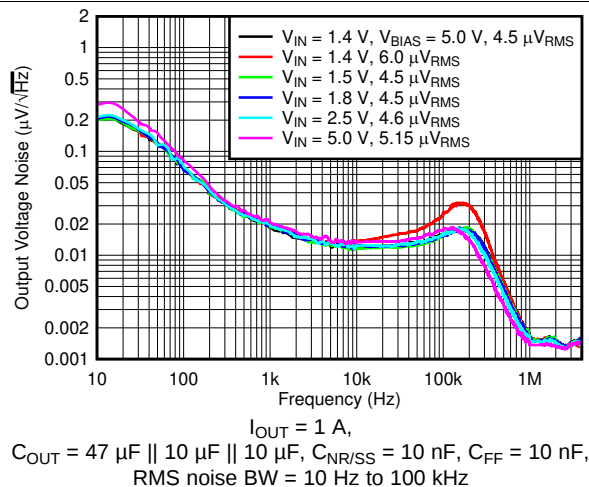
图 11. Output Noise vs Frequency and Input Voltage
