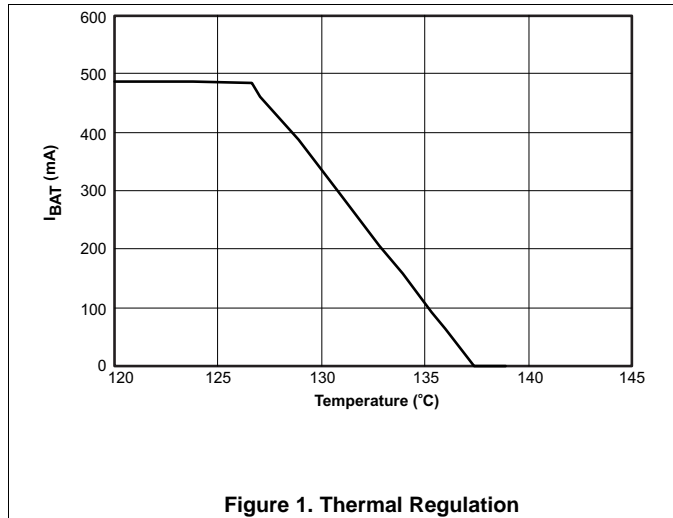
Figure 1. Thermal Regulation
