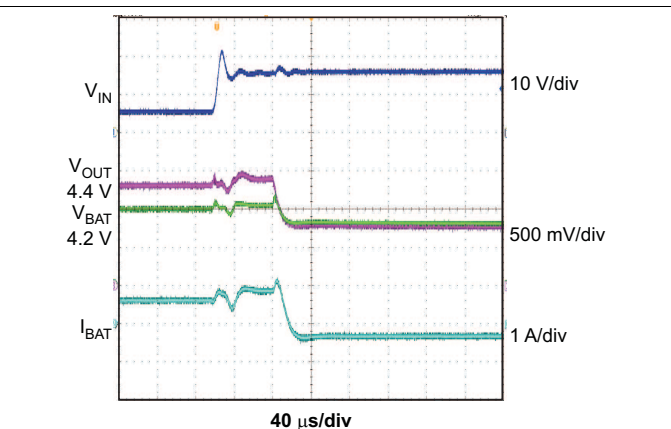
Figure 34. OVP Fault
