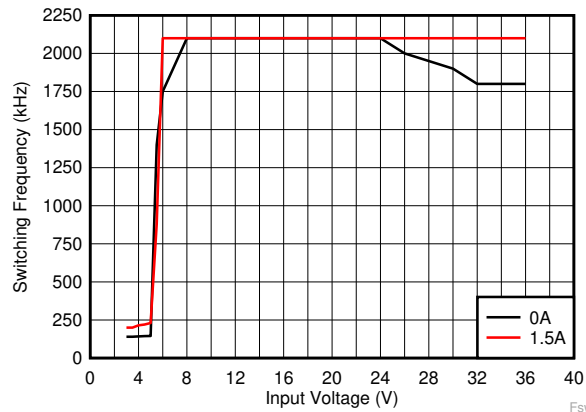
LM63615 V_{OUT} = 5\text{ V} f_{SW} = 2100\text{ kHz} (FPWM)
