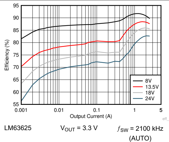
图 9-13. Efficiency
