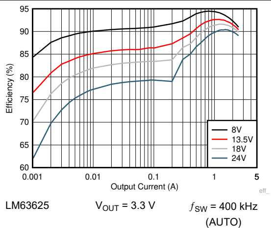
图 9-12. Efficiency
