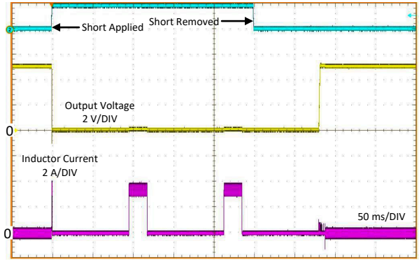
图 8-14. Short-Circuit Transient and Recovery; LM63625
