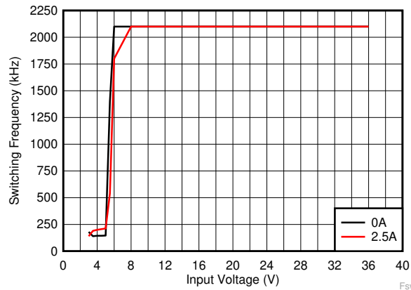
LM63625 V_{OUT} = 5\text{ V} f_{SW} = 2100\text{ kHz} (FPWM)
