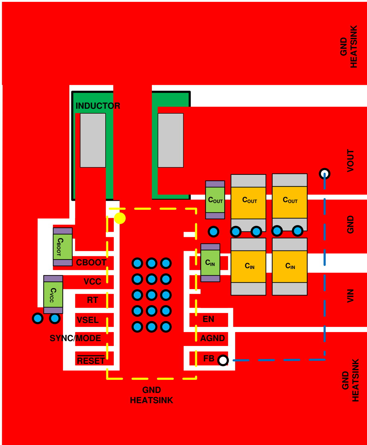
图 11-2. Example Layout for HTSSOP Package
