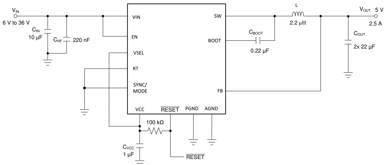
图 9-1. Example Application Circuit V_{IN} = 12\text{ V} , V_{OUT} = 5\text{ V} , I_{OUT} = 2.5\text{ A} , f_{SW} = 2.1\text{ MHz}
