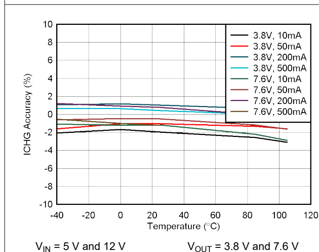
图 6-5. ICRG Accuracy vs. Temperature
