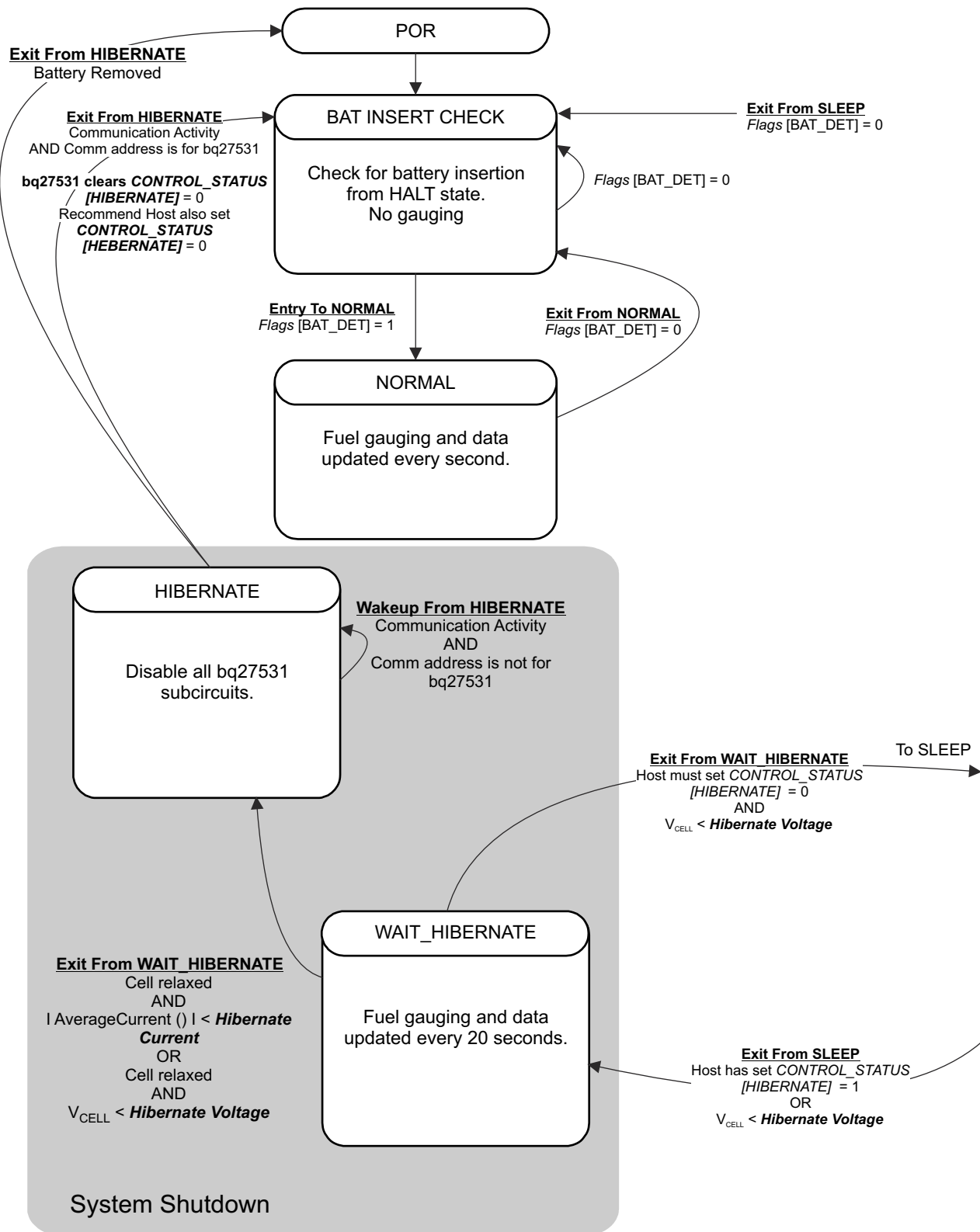
图 8-2. Power Mode Diagram—System Shutdown
