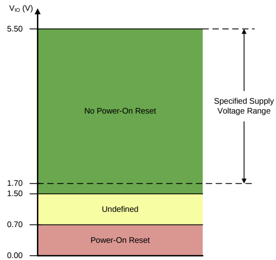
Figure 63. Threshold Levels for V_{IO} POR Circuit
