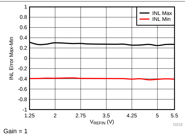
Figure 18. Integral Linearity Error vs Reference Voltage
