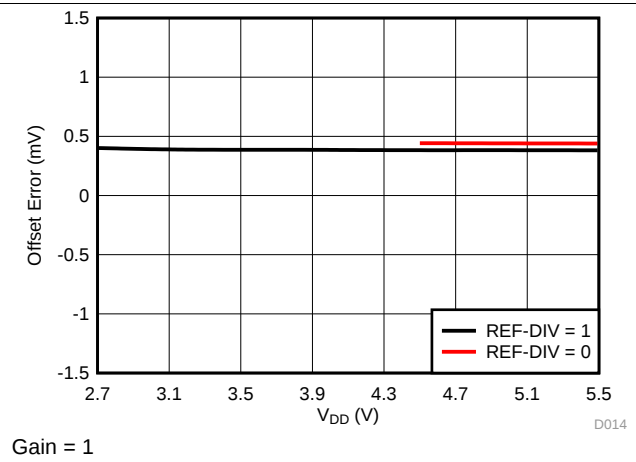
Figure 14. Offset Error vs Supply Voltage
