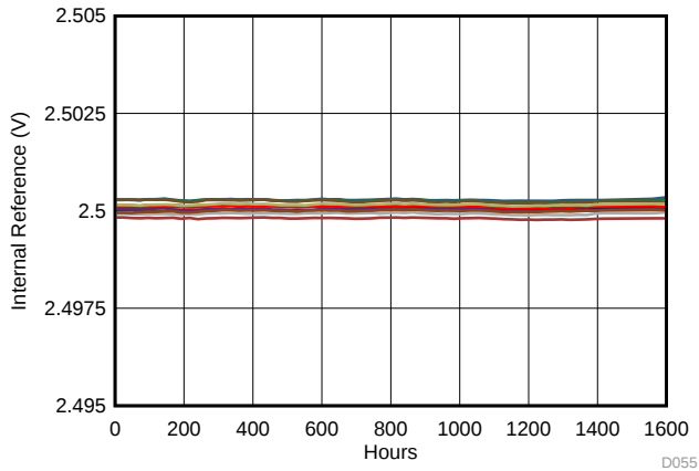
Figure 55. Internal Reference Voltage vs Time
