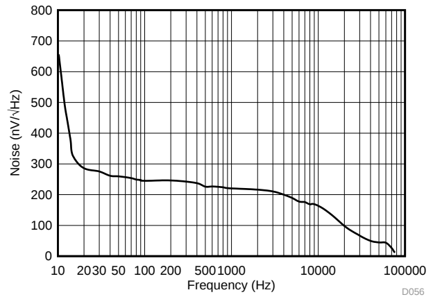
Figure 56. Internal Reference Noise Density vs Frequency
