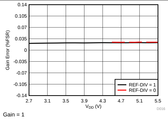
Figure 16. Gain Error vs Supply Voltage
