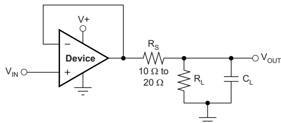
Figure 38. 改进容性负载驱动
