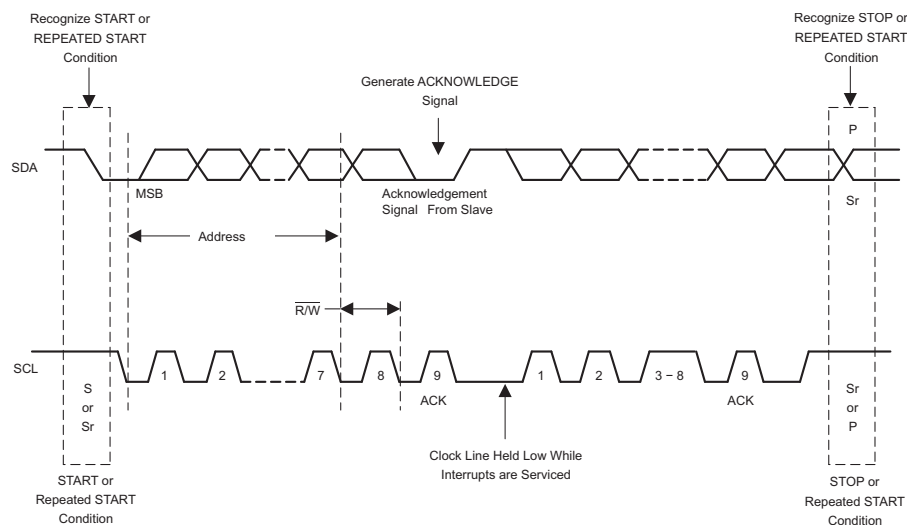
Figure 7-23. Bus Protocol
