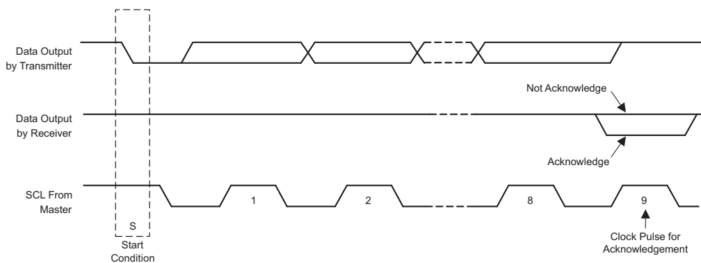
Figure 7-22. Acknowledge on the I 2 C Bus
