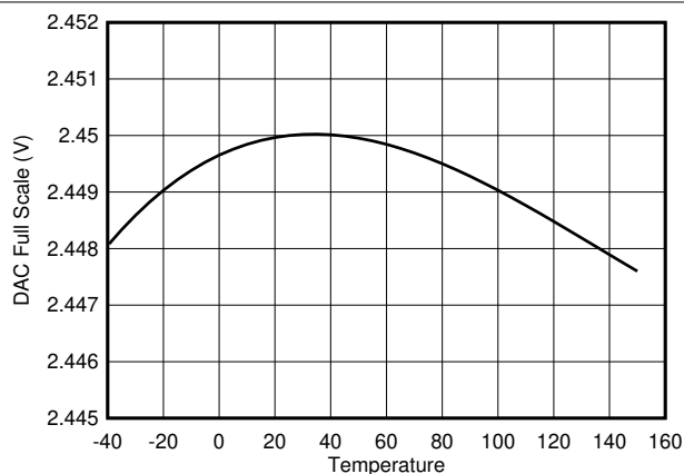
图 6-16. DAC Full Scale vs Temperature
