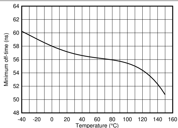
图 6-18. Minimum Off-time vs Temperature
