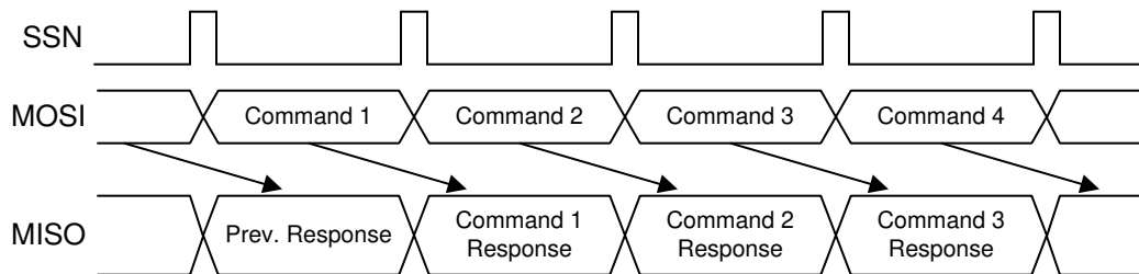
图 7-15. SPI Command and Response Sequence
