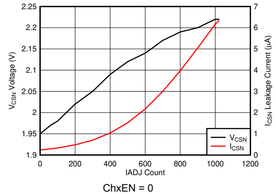
图 6-4. CSN Voltage and Leakage Current vs IADJ Count
