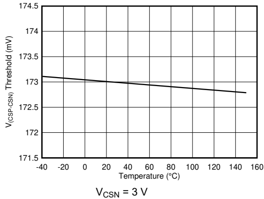
图 6-1. V_{(CSP - CSN)} Current Sense Threshold vs Temperature
