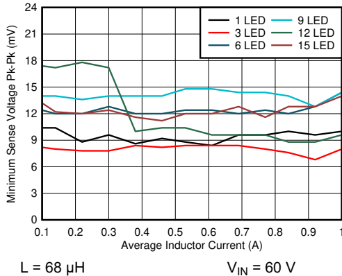
图 6-5. Minimum Ripple Voltage vs Average Inductor Current
