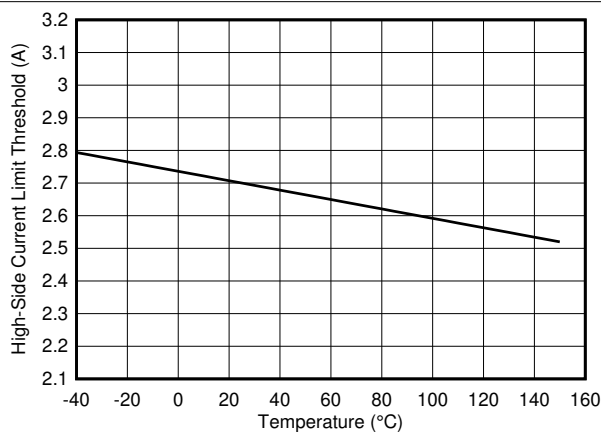
图 6-11. High-Side Current Limit Threshold vs Temperature
