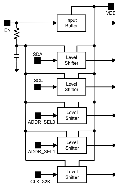
Figure 20. Using EN Pin as Digital IO Voltage Reference
