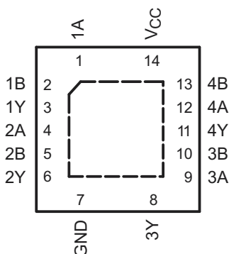
SN74AHCT86 . . . RGY PACKAGE (TOP VIEW)
