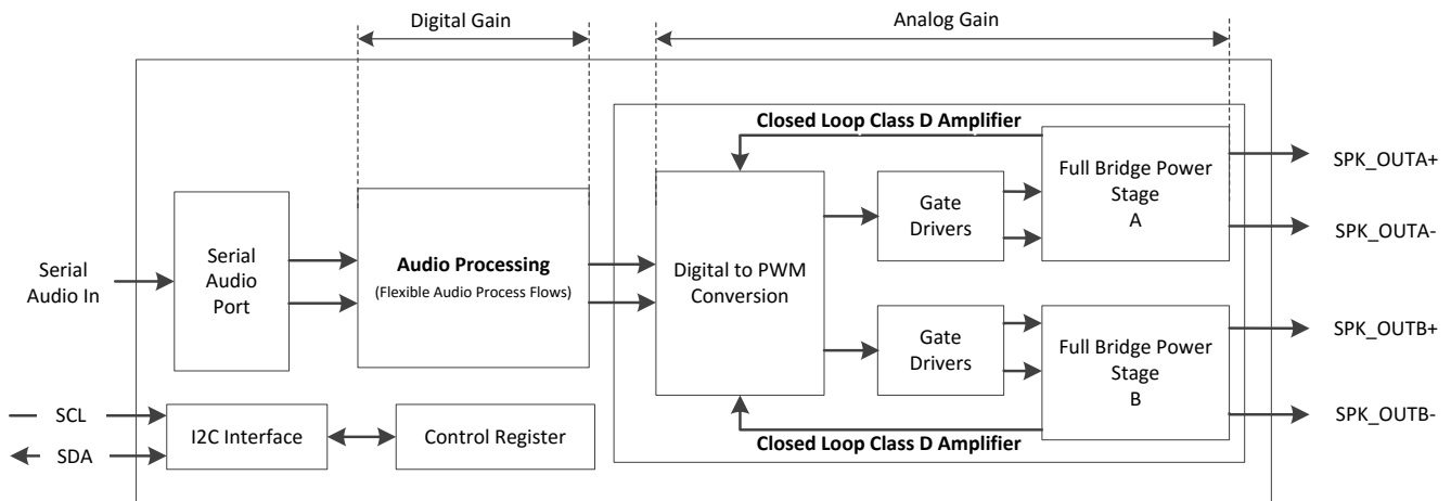
图 61. Speaker Amplifier Gain
