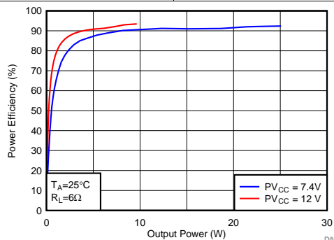
图 40. Efficiency vs Output Power
