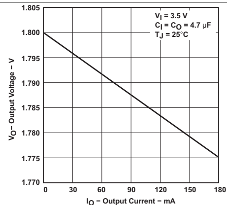
Figure 2. TPS76318-Q1 Output Voltage vs Output Current
