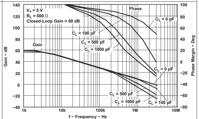
Figure 24. Gain and Phase Margin vs Frequency
