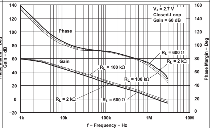
Figure 22. Gain and Phase Margin vs Frequency
