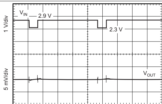
Figure 19. Line Transient Response
