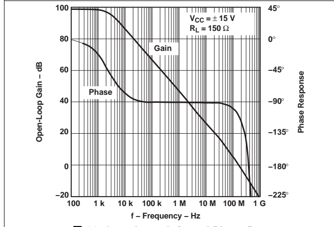
图 11. Open-Loop Gain and Phase Response
