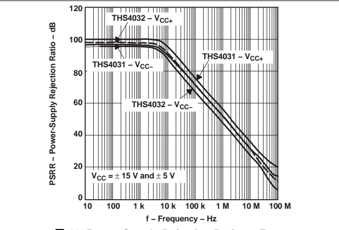
图 12. Power-Supply Rejection Ratio vs Frequency
