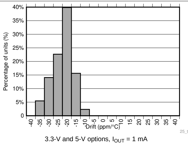
图 11. Temperature Drift Histogram (25°C to 150°C)
