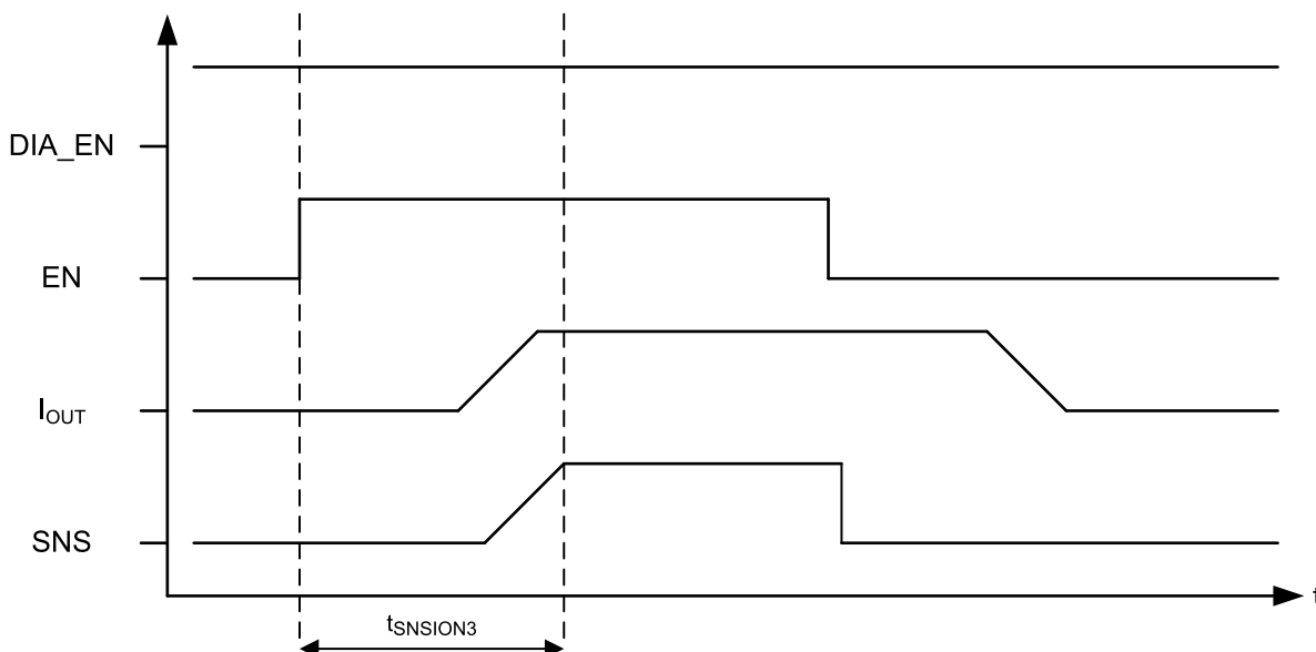
图 13. Current Sensing in Low-Duty Cycle Applications
