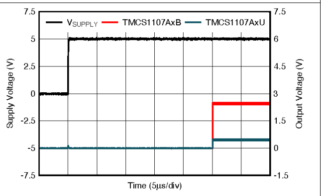
图 7-12. Startup Transient Response
