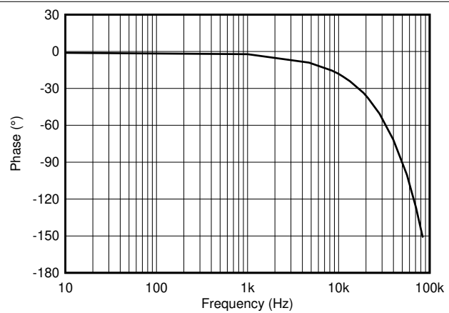
图 7-4. Phase vs. Frequency, All Gains
