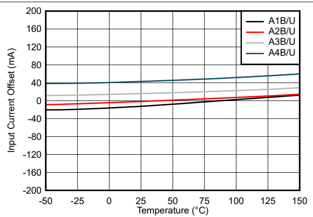
图 7-2. TMCS1107 Input Offset Current vs. Temperature
