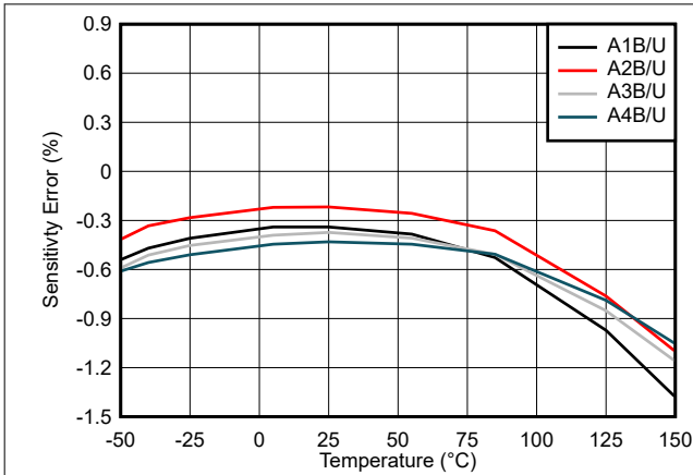
图 7-1. TMCS1107 Sensitivity Error vs. Temperature
