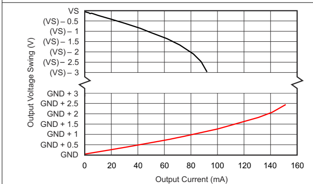
图 7-5. Output Swing vs. Output Current
