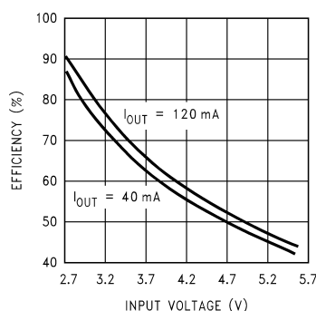
Figure 14. Power Efficiency
