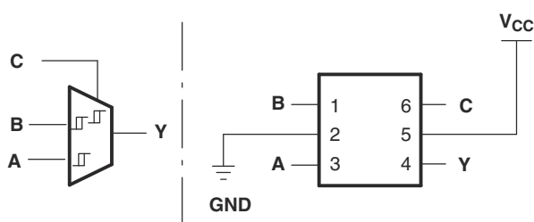
图 7-4. 157: 2-to-1 Data Selector/MUX When C is L, Y = B When C is H, Y = A
