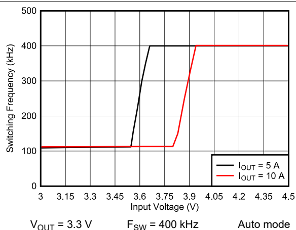
图 9-26. Frequency Dropout
