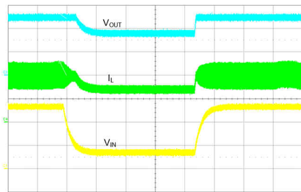
V_{OUT} = 5\text{ V} F_{SW} = 2100\text{ kHz} FPWM mode I_{OUT} = 4\text{ A} V_{IN} = 13.5\text{ V to } 4\text{ V to } 13.5\text{ V}
