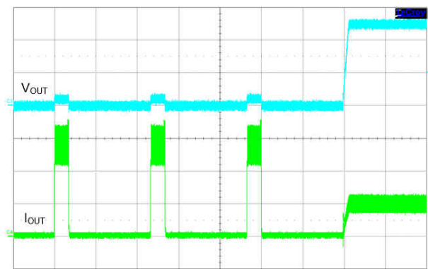
V_{OUT} = 5\text{ V} F_{SW} = 2100\text{ kHz} FPWM mode I_{OUT} = \text{Short Circuit to } 5\text{ A} V_{IN} = 13.5\text{ V}
