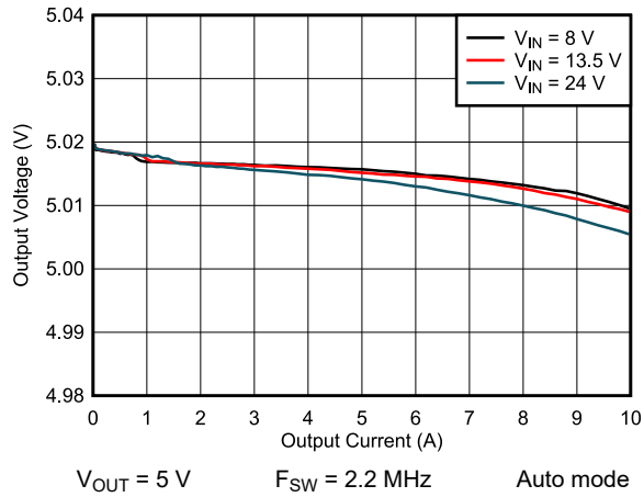
图 9-17. Load and Line Regulation
