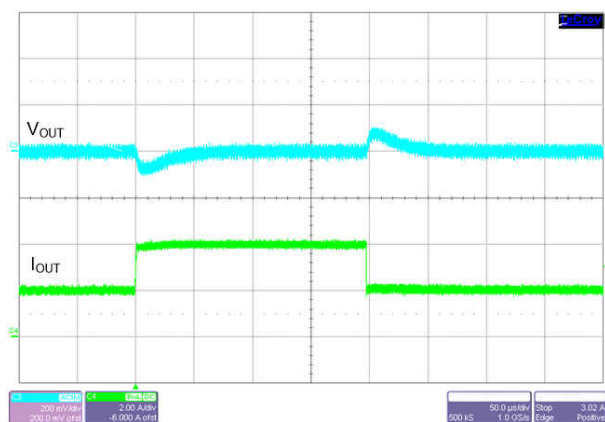
V_{OUT} = 5\text{ V} F_{SW} = 400\text{ kHz} Auto mode I_{OUT} = 2\text{ A to } 4\text{ A to } 2\text{ A} V_{IN} = 13.5\text{ V} T_R = T_F = 1\text{ }\mu\text{s}
