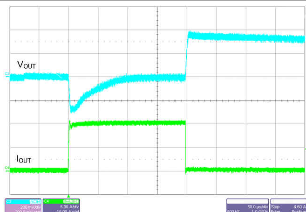
V_{OUT} = 5\text{ V} F_{SW} = 400\text{ kHz} Auto mode I_{OUT} = 10\text{ mA to } 10\text{ A} V_{IN} = 13.5\text{ V} T_R = T_F = 1\text{ }\mu\text{s}
