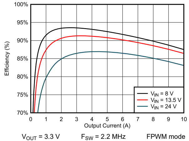
图 9-12. Efficiency
