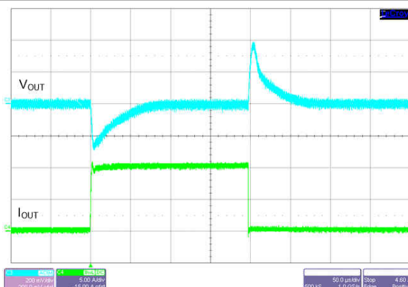
V_{OUT} = 5\text{ V} F_{SW} = 400\text{ kHz} FPWM mode I_{OUT} = 10\text{ mA to } 10\text{ A} V_{IN} = 13.5\text{ V} T_R = T_F = 1\text{ }\mu\text{s}
