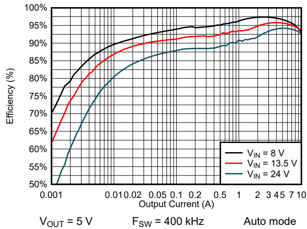
图 9-5. Efficiency
