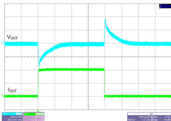
V_{OUT} = 5\text{ V} F_{SW} = 400\text{ kHz} Auto mode I_{OUT} = 5\text{ A to } 10\text{ A to } 5\text{ A} V_{IN} = 13.5\text{ V} T_R = T_F = 1\text{ }\mu\text{s}
