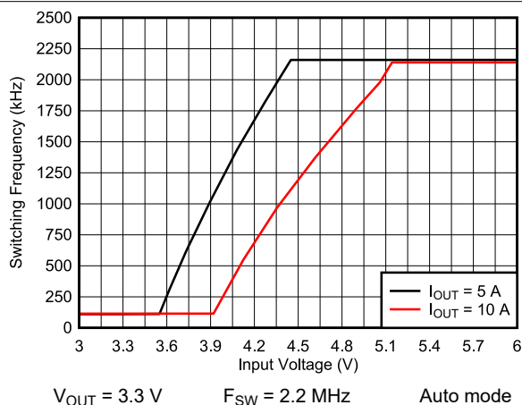
图 9-28. Frequency Dropout
