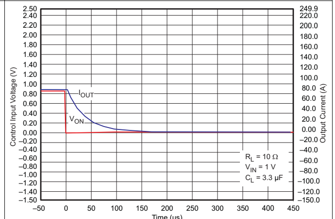
Figure 51. t_{OFF} Response
