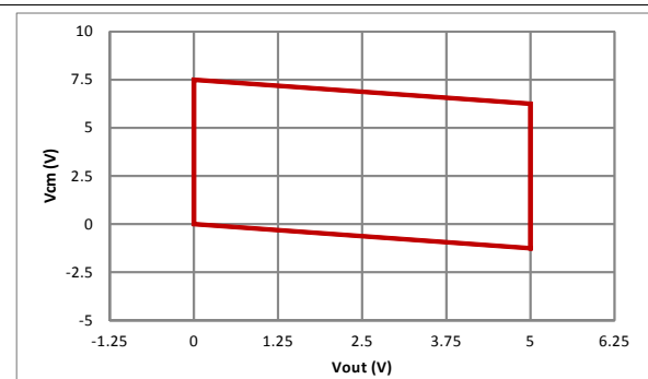
图 68. Input Common-Mode Voltage vs Output Voltage G = 2 , Bipolar Supply
