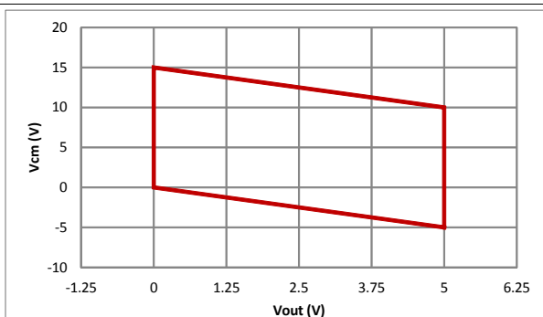
图 67. Input Common-Mode Voltage vs Output Voltage G = 1/2 , Bipolar Supply
