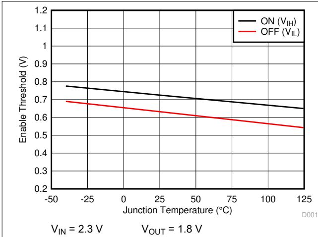
图 6-1. V_{EN} Threshold vs Temperature
