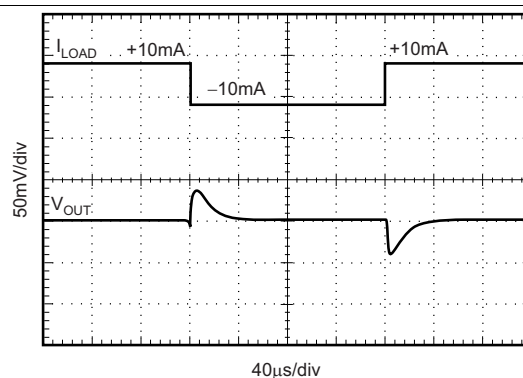
Figure 16. Load Transient C_L = 1\text{ μF} , \pm 10\text{-mA} Output Pulse
