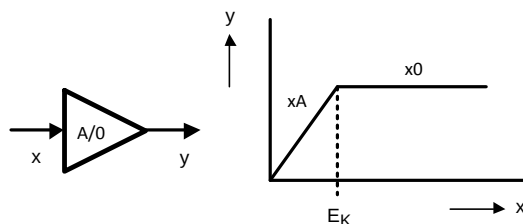
Figure 73. Gain Cell
