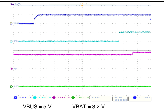
图 43. Power Up with Charge Disabled
