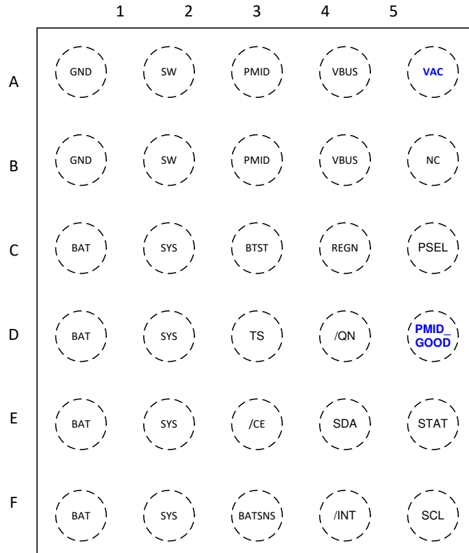
BQ25618 YFF Package 30-Pin WCSP Top View
