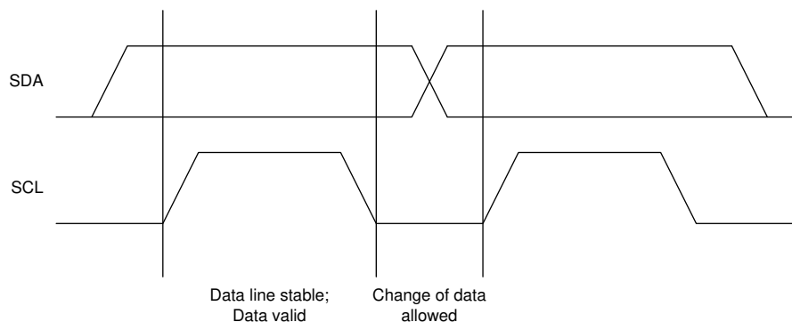
图 17. Bit Transfer on the I 2 C Bus
