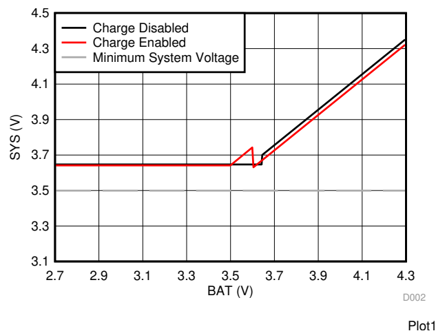
图 12. System Voltage vs Battery Voltage
