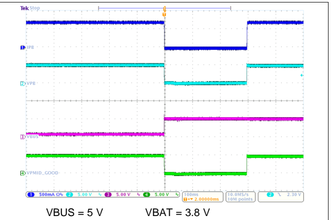
图 41. VBUS Plugged In with Boost Mode Enabled
