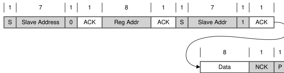
图 22. Single Read
