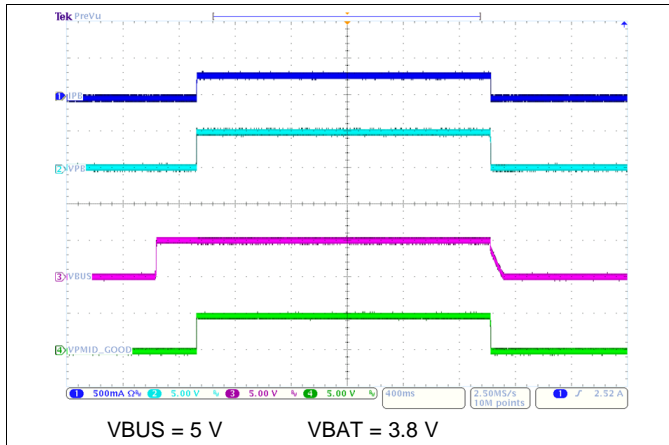
图 40. VBUS Plugged In and Unplugged with Boost Mode Disabled
