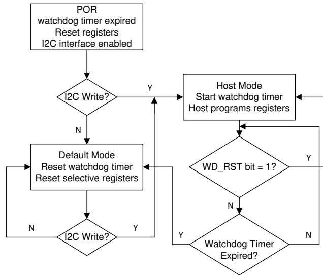
图 25. Watchdog Timer Flow Chart
