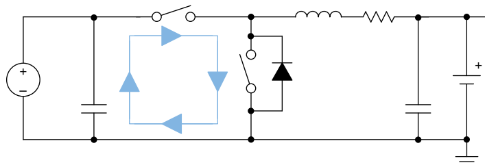
图 49. High Frequency Current Path
