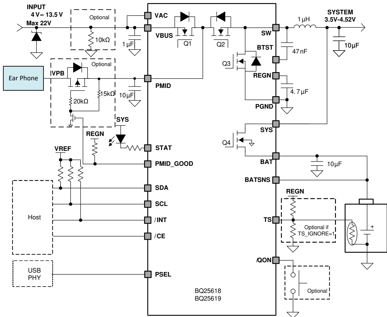
图 39. BQ25619 Application Diagram with Optional PMOS
