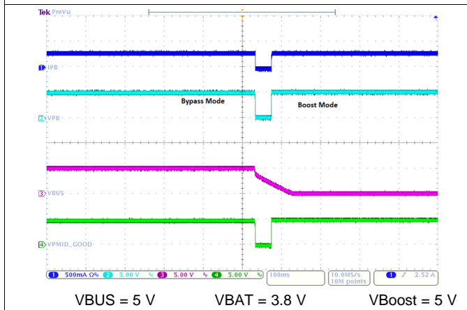
图 42. VBUS Unplugged with Boost Mode Enabled
