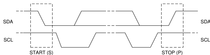
图 18. TS START and STOP conditions
