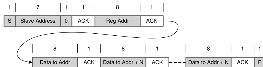
图 23. Multi-Write
