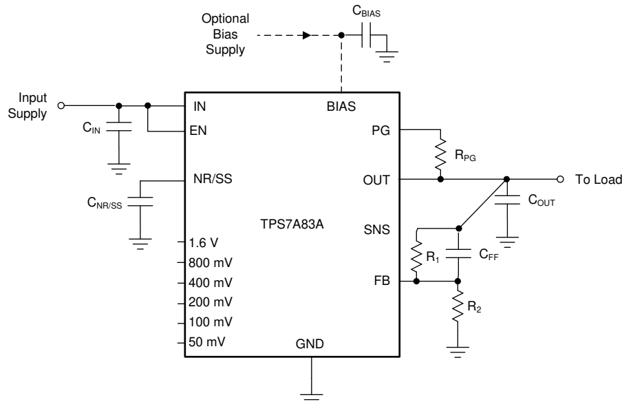
图 9-1. Adjustable Operation
