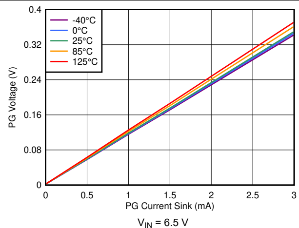
图 7-41. PG Voltage vs PG Current Sink
