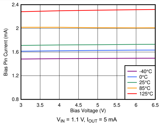
图 7-33. BIAS Pin Current vs Bias Voltage
