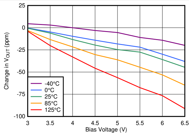
图 7-28. Load Regulation (5-V Output)
