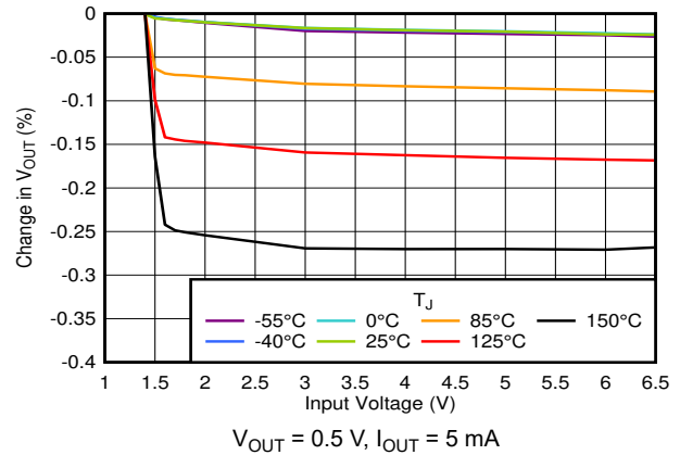
图 7-54. Line Regulation vs V_{IN}
