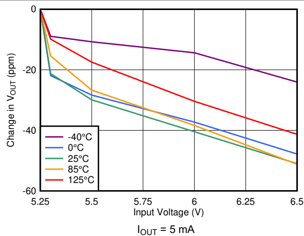
图 7-31. Line Regulation (5-V Output)
