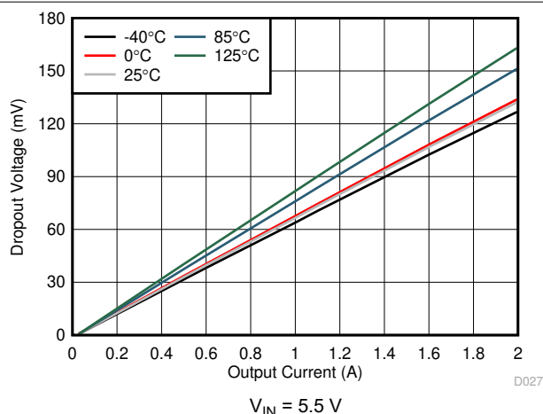
图 7-50. Dropout Voltage vs Output Current (High V_{IN} )
