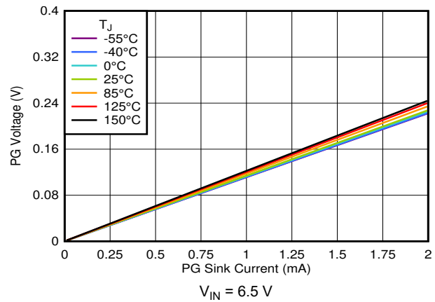
图 7-66. PG Voltage vs PG Current Sink
