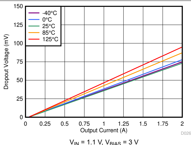
图 7-49. Dropout Voltage vs Output Current With BIAS
