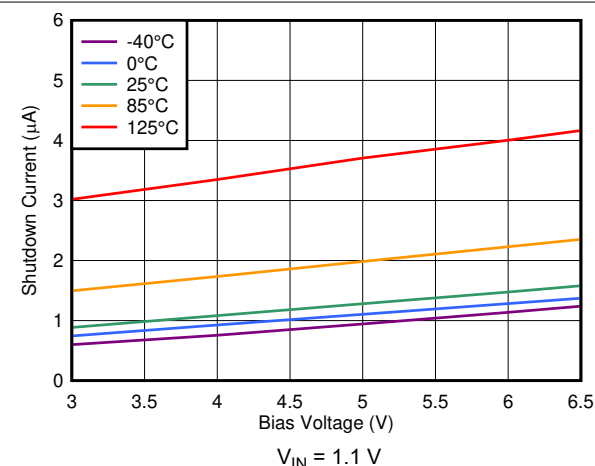
图 7-35. Shutdown Current vs Bias Voltage
