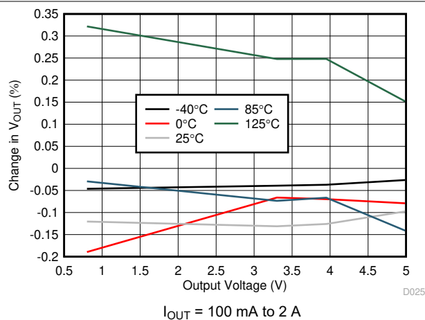
图 7-25. Load Regulation vs Output Voltage
