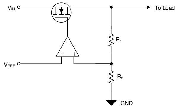
图 8-1. Simplified Regulation Circuit
