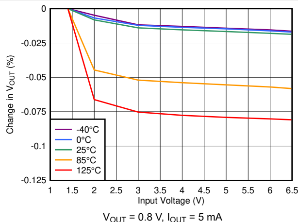
图 7-29. Line Regulation
