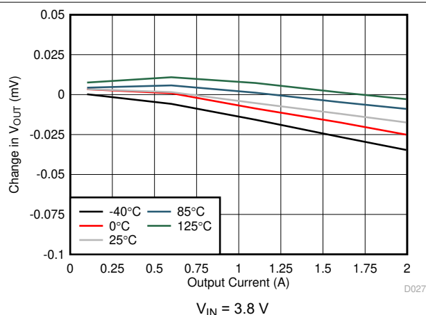
图 7-27. Load Regulation (3.3-V Output)
