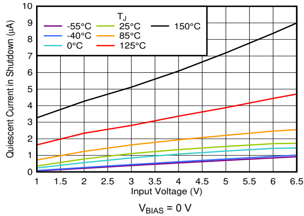
图 7-59. Shutdown Current vs Input Voltage
