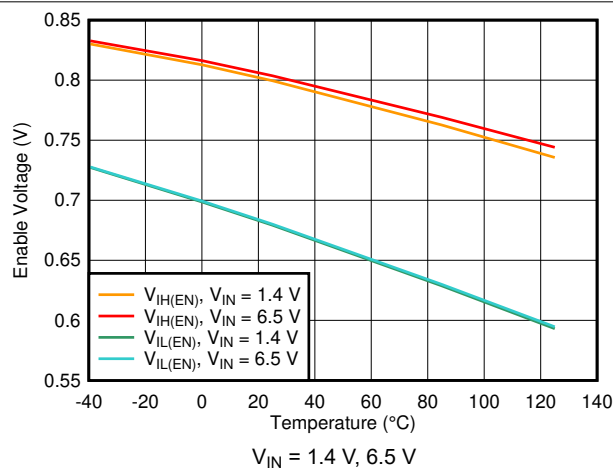
图 7-39. Enable Threshold vs Temperature
