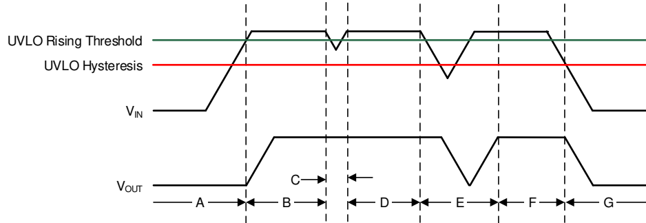
图 9-4. Typical UVLO Operation
