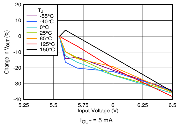
图 7-56. Line Regulation vs V_{IN} (5.2-V Output)
