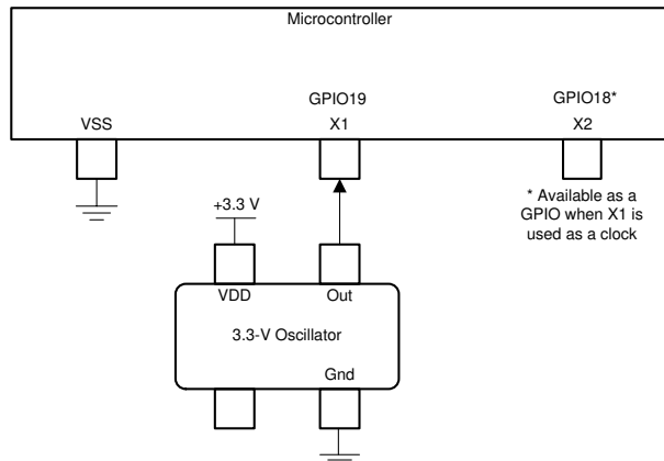
图 7-12. Single-ended 3.3-V External Clock
